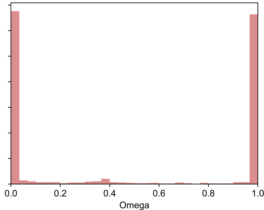
BUIP - Advanced
