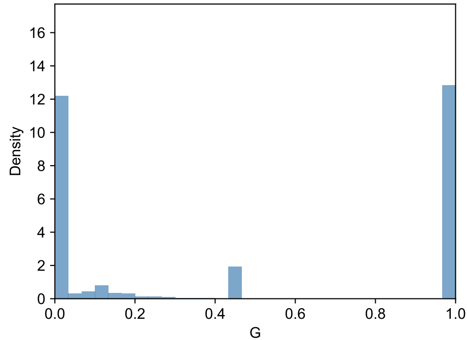
STR - Complete Sample
