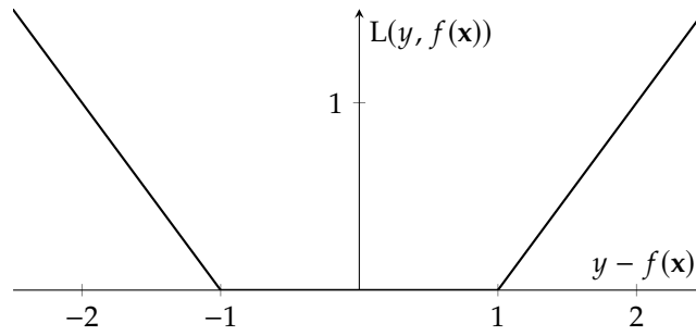
Figure 5.2 \epsilon -insensitive loss function with \epsilon = 1 .
