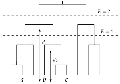
Figure 7.1 Example of a dendrogram. a , b and c are three observations.
