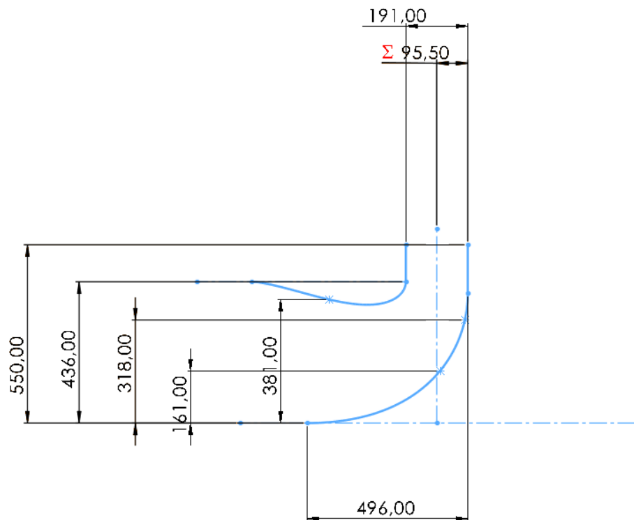
Figura 2 corona-mozzo Solidworks
