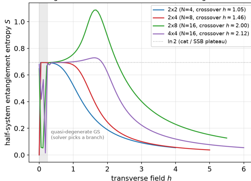
Entanglement across the transition — rectangular lattices
