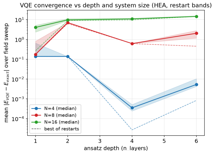
HEA depth scan: deeper = worse at N = 16
