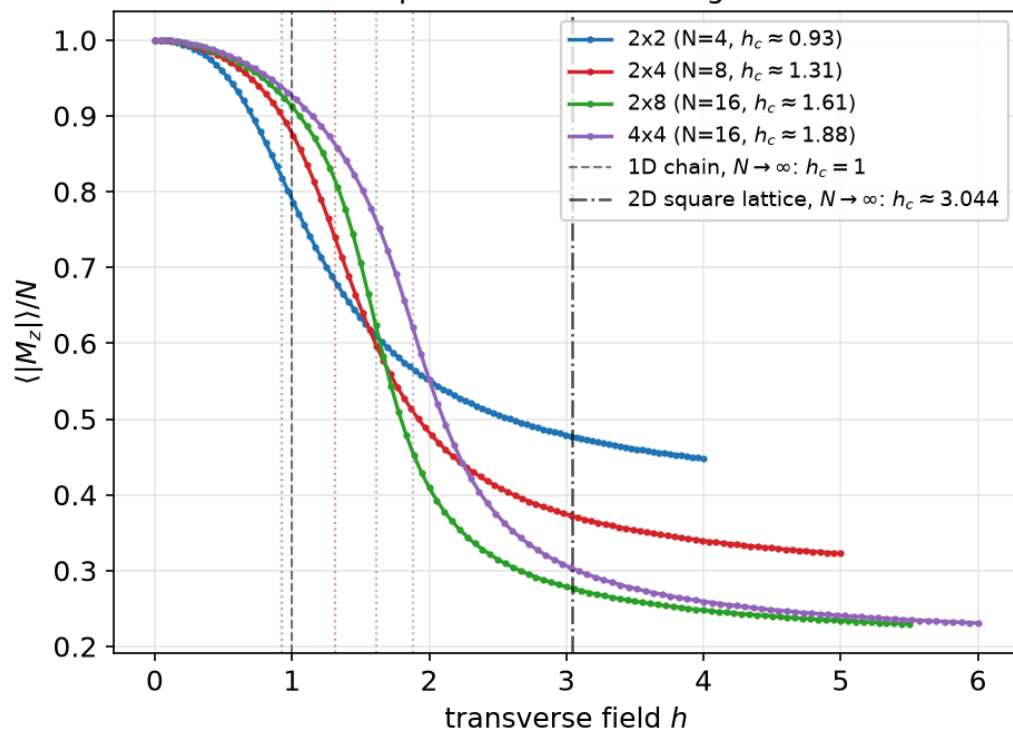
TFIM order parameter — rectangular lattices
