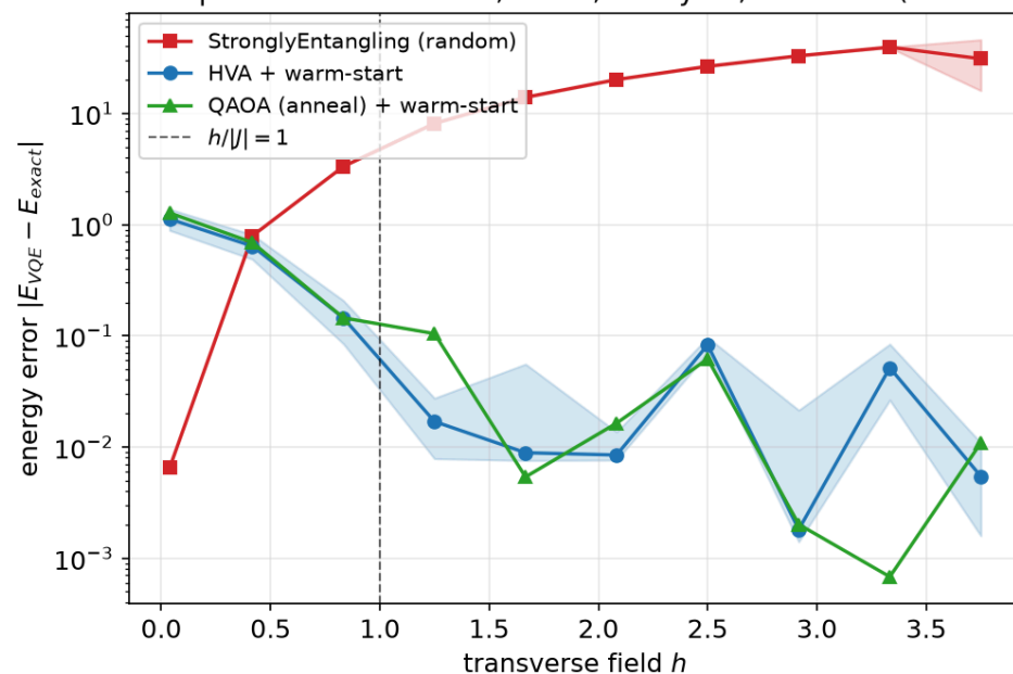
Ansatz comparison — TFIM chain, N=16 , 10 layers, 4 restarts (median \pm IQR)
