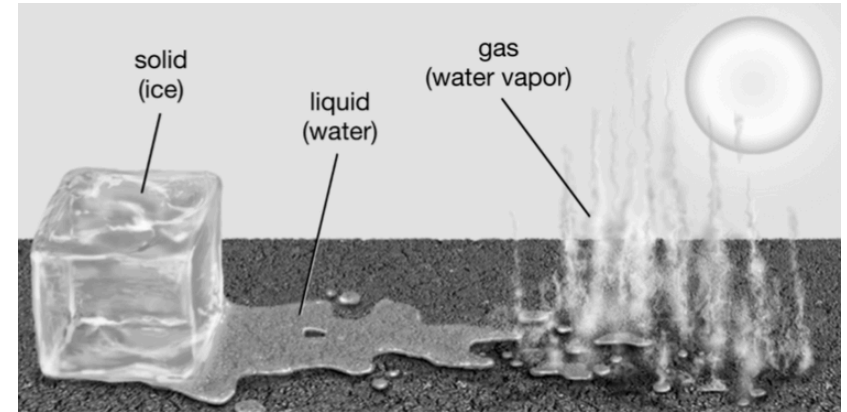
First-order: ice → water → vapor
