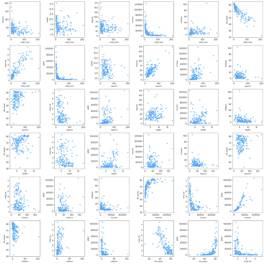
Figure 3: Pairwise scatterplot.
