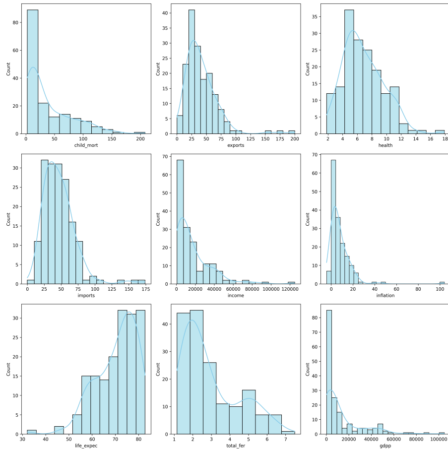
Figure 1: Columns distribution of X and Y, after a transformation.
