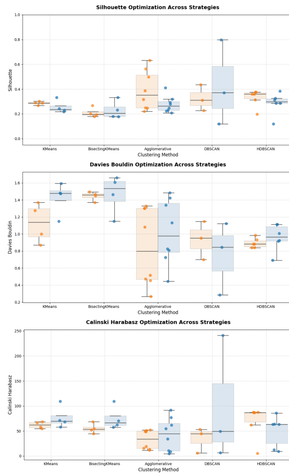
Figure 5: Clustering Evaluation
