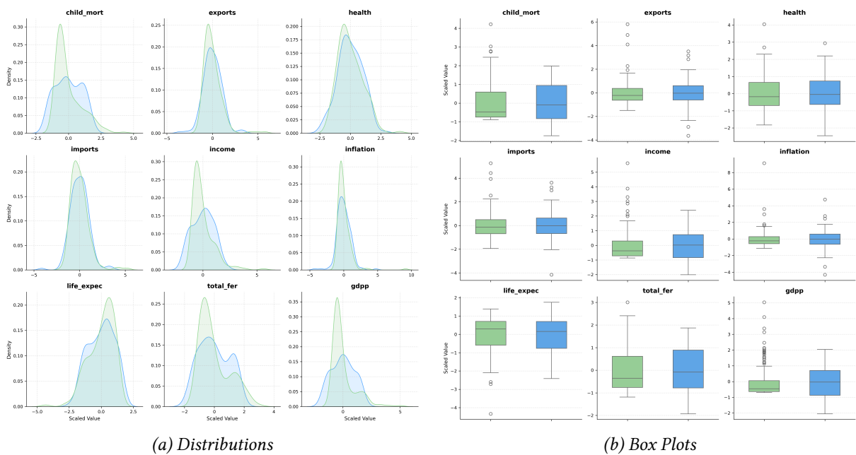
Figure 4: Comparison
