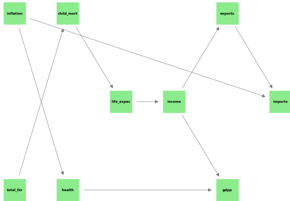
Figure 6: Directed Acyclic Graph builded using PC
