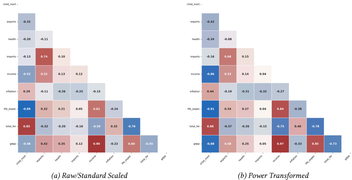
Figure 3: Correlations
