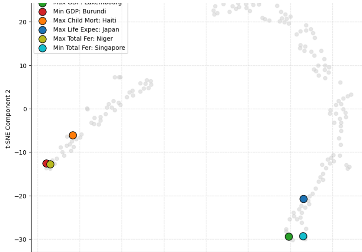
Figure 1: t-SNE (perplexity = 10)
