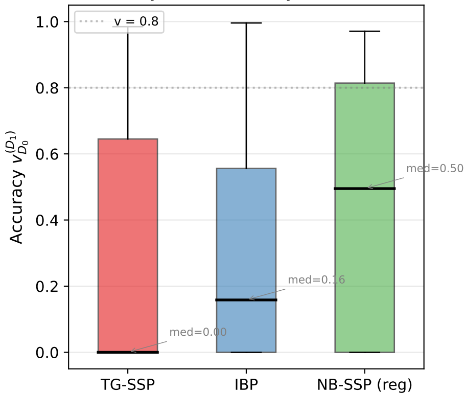
ASOS: Accuracy distribution by method (144 arms)
