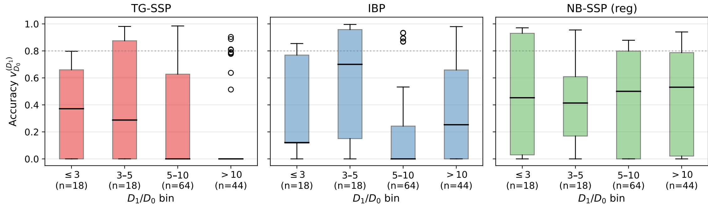
ASOS: Accuracy stratified by extrapolation ratio
