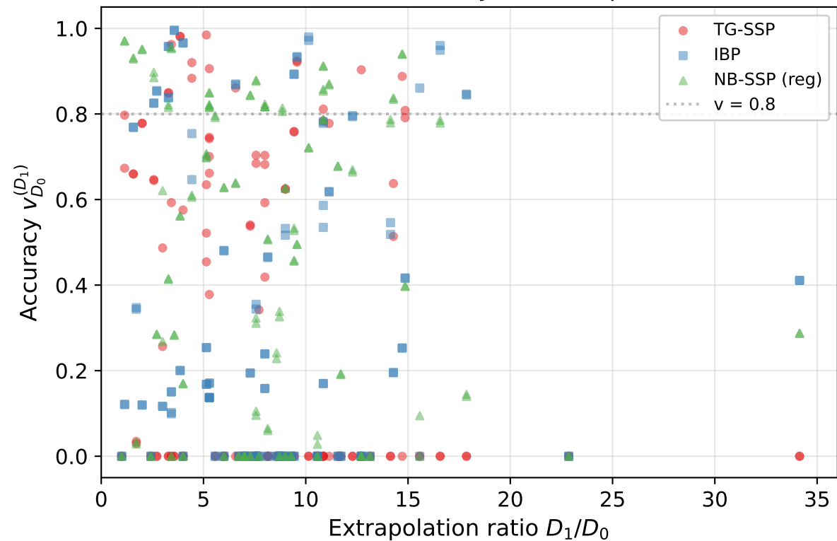
ASOS: Prediction accuracy vs. extrapolation ratio
