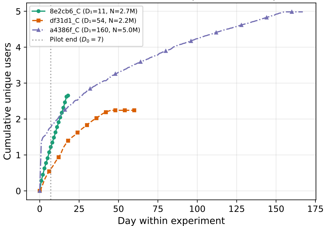
ASOS: Cumulative new users (3 representative experiments)
