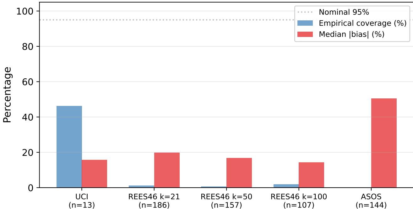
CI Coverage vs. Bias Across Datasets (NB-SSP reg, 95% nominal)
