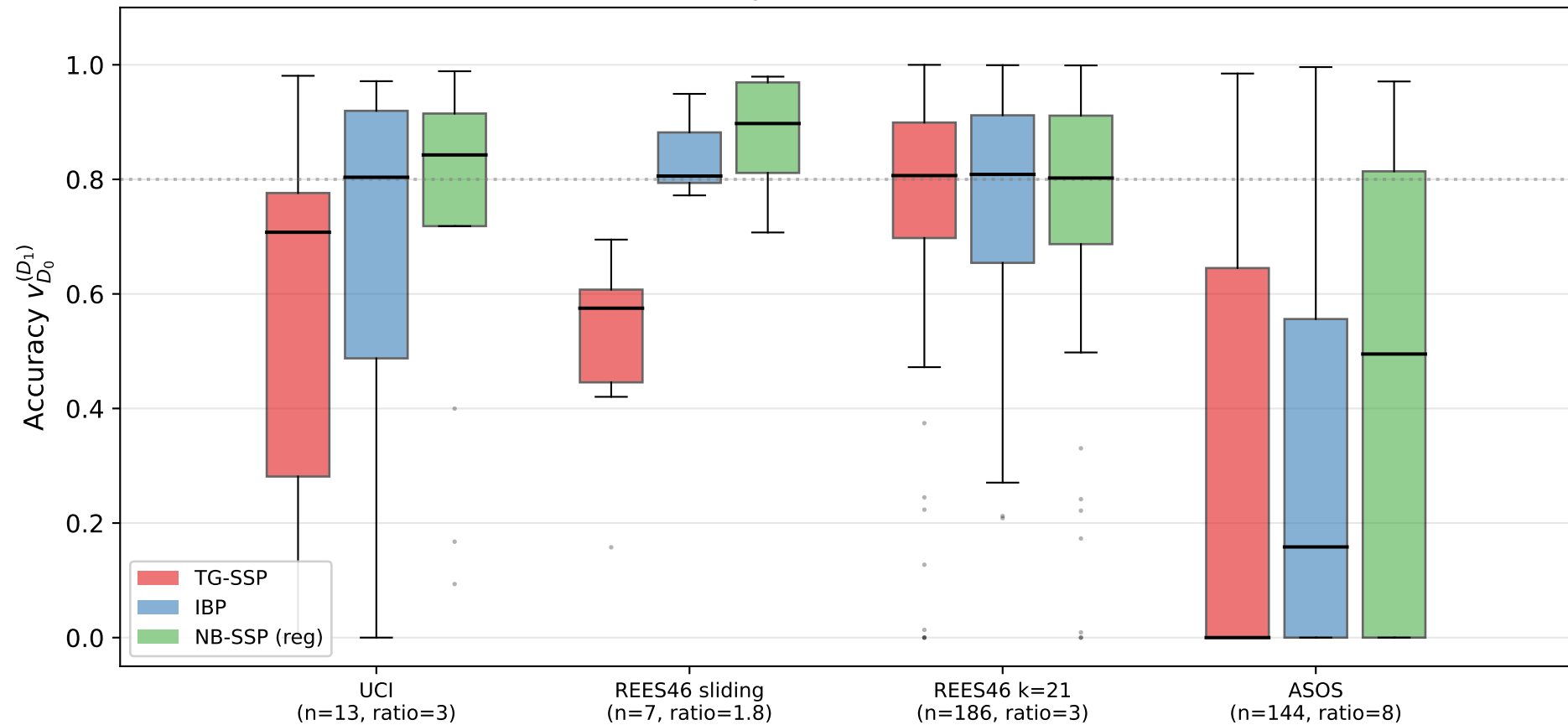
Prediction accuracy across datasets and methods
