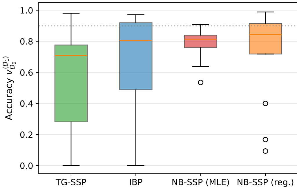
New user prediction accuracy (UCI Online Retail)
