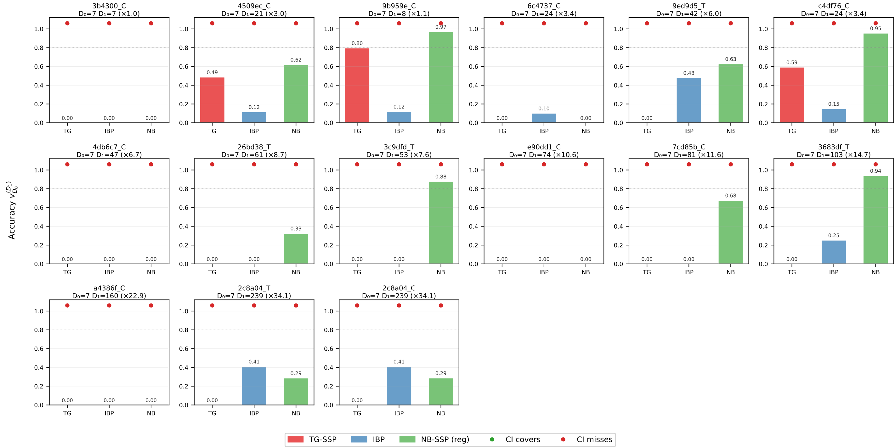
ASOS — selected arms (15 of 144), stratified by extrapolation ratio
