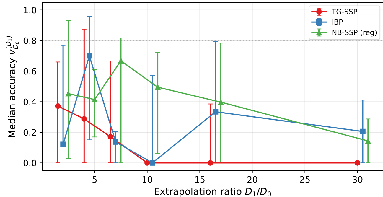
ASOS: Accuracy vs. extrapolation ratio (median \pm IQR)
