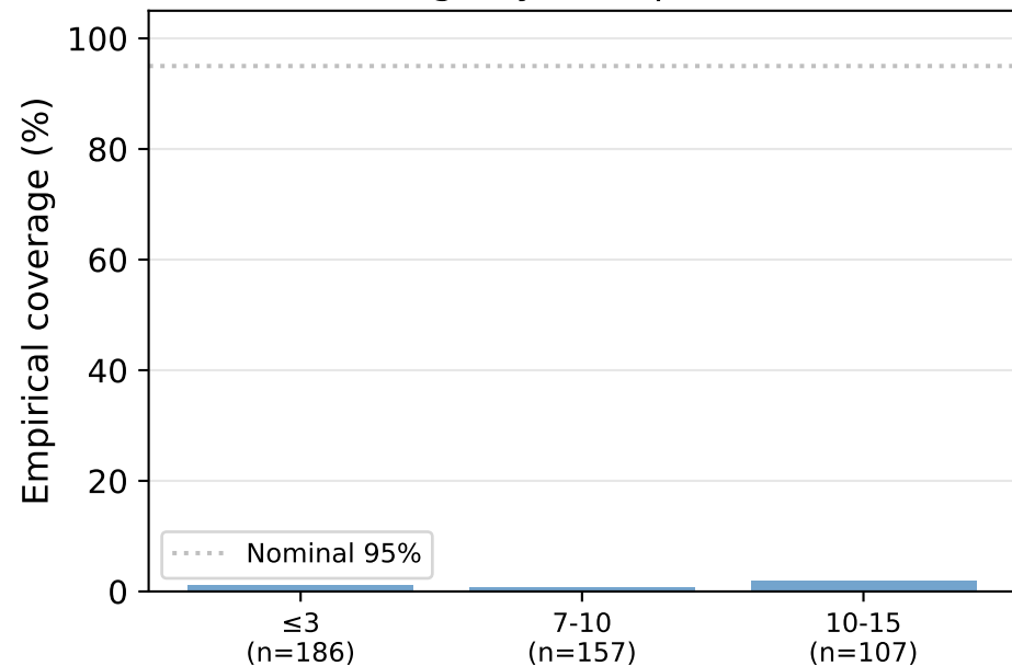
CI Coverage by Extrapolation Ratio
