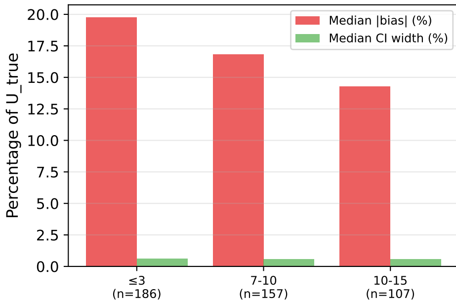
Bias vs. CI Width
