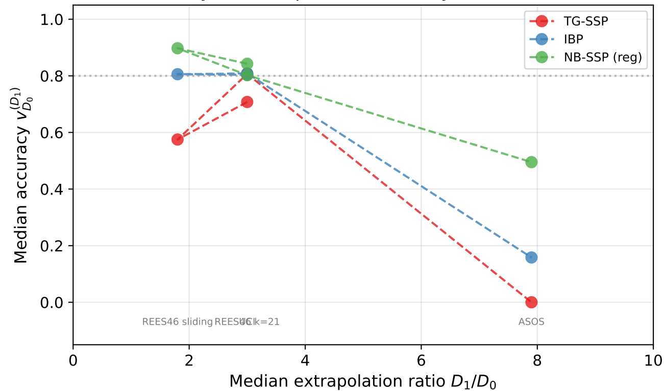
Accuracy vs. extrapolation difficulty across datasets
