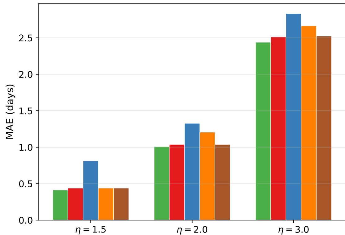
REES46 k = 100 (107 windows)
