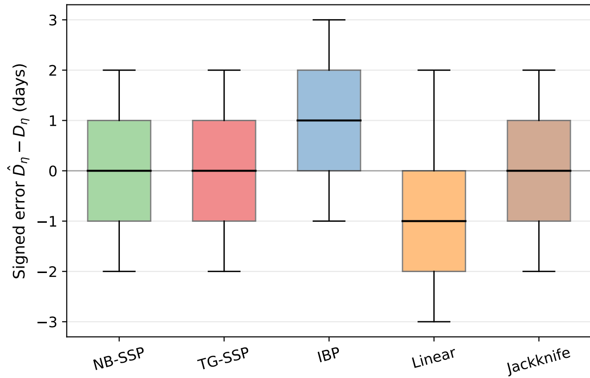
REES46 k = 100 (107 windows), \eta = 2.0
