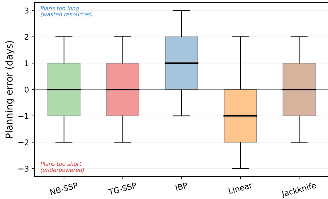
REES46 k = 100 ( \eta = 2 )
