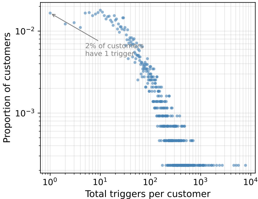
Distribution of per-customer trigger counts
