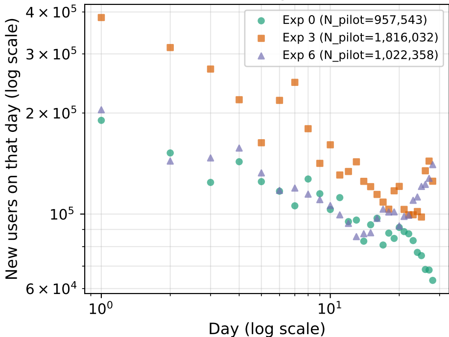
REES46: Power-law decay of new user arrivals
