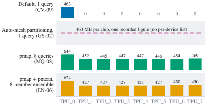
(b) HBM in use per chip (MB)
