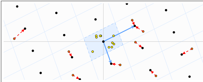
Figure 38: Reducing a number of hashed messages H(\mathbf{m}) to the origin
