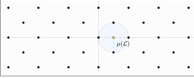
Figure 20: The “hexagonal” lattice and its covering radius
