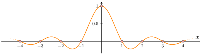
Figure 107: The \text{sinc}(x) function
