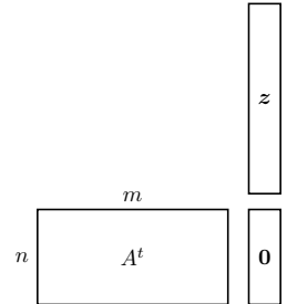
Figure 48: Shape of the matrices used in SIS
