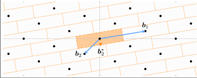
Figure 32: A lattice and its Babai’s fundamental region
