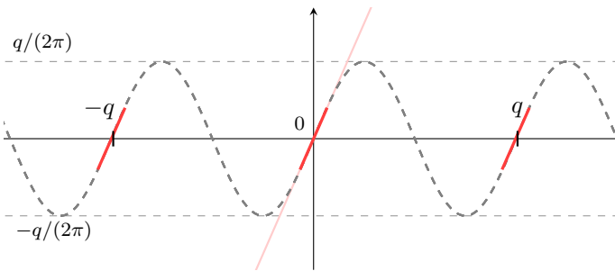
Figure 62: The modular reduction by q , in red, can be approximated by a sine function if the input is not too far from a multiple of q
