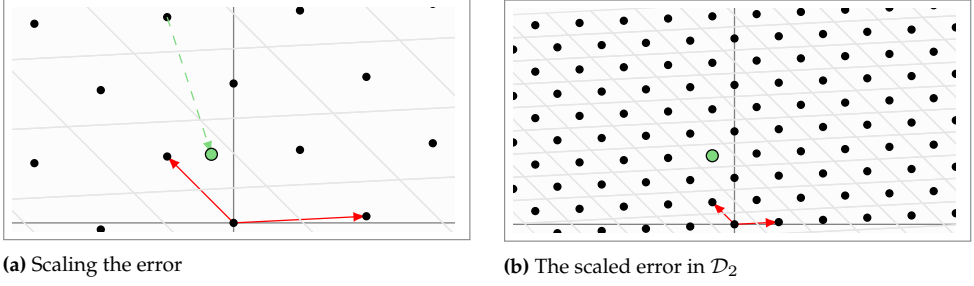
Figure 68: Given a “rounded” ciphertext in q_1/q_2\mathcal{D}_2 , we can scale it down by the factor q_1/q_2
