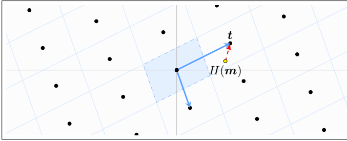
Figure 37: Some hashed message H(\mathbf{m}) and its closest lattice point \mathbf{t}
