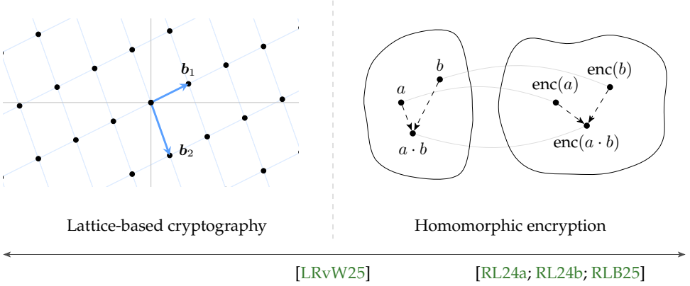
Figure 9: Summary of the topics and contributions that will be discussed in this thesis. The works are positioned in a spectrum that goes from lattice-based cryptography to homomorphic encryption
