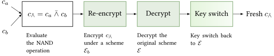
Figure 7: High-level overview of a simple bootstrapping framework inspired from [DM15]. Green boxes refer to \mathcal{E}_b , while the others to \mathcal{E}
