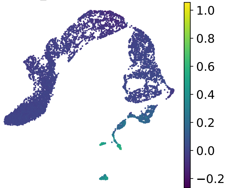
MEA_score downsampled
