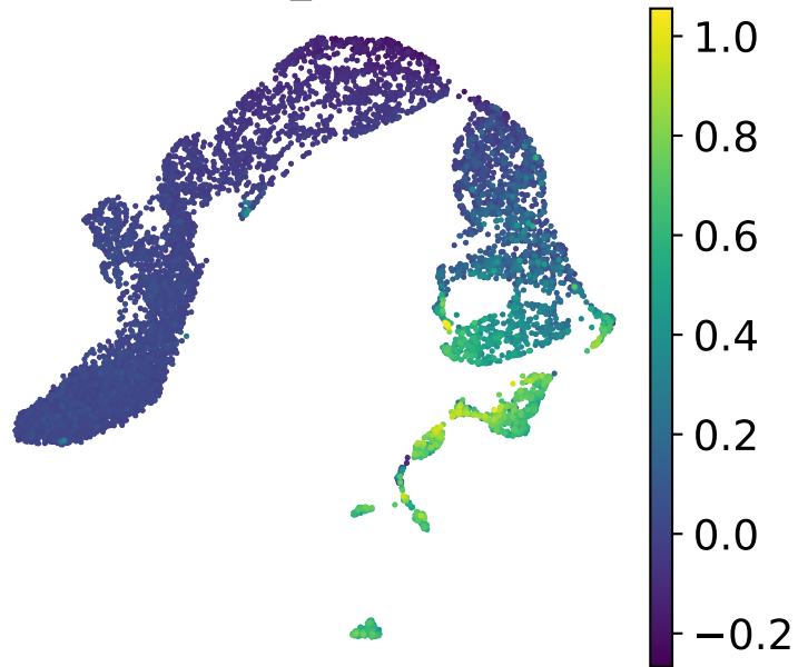
SEG_score
