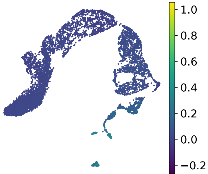
MEA_score
