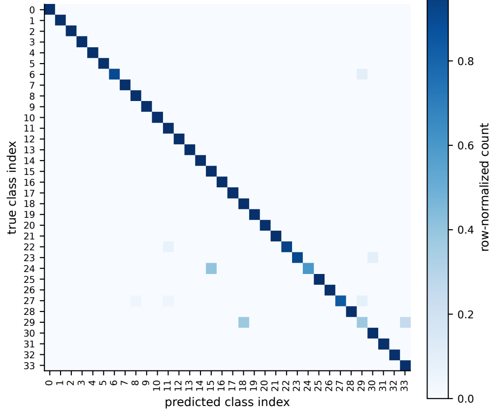
Contrastive emb = 3 (Macro-F1 = 0.950)
