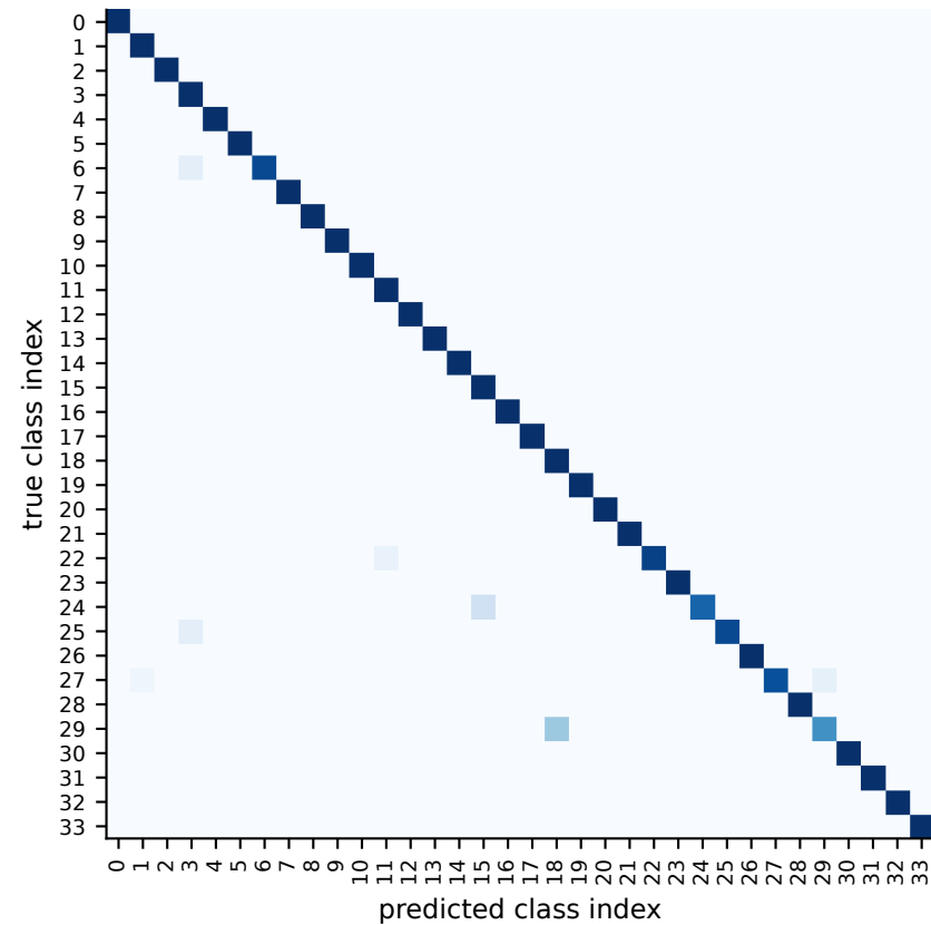
VMGP d = 96 (Macro-F1 = 0.970)
