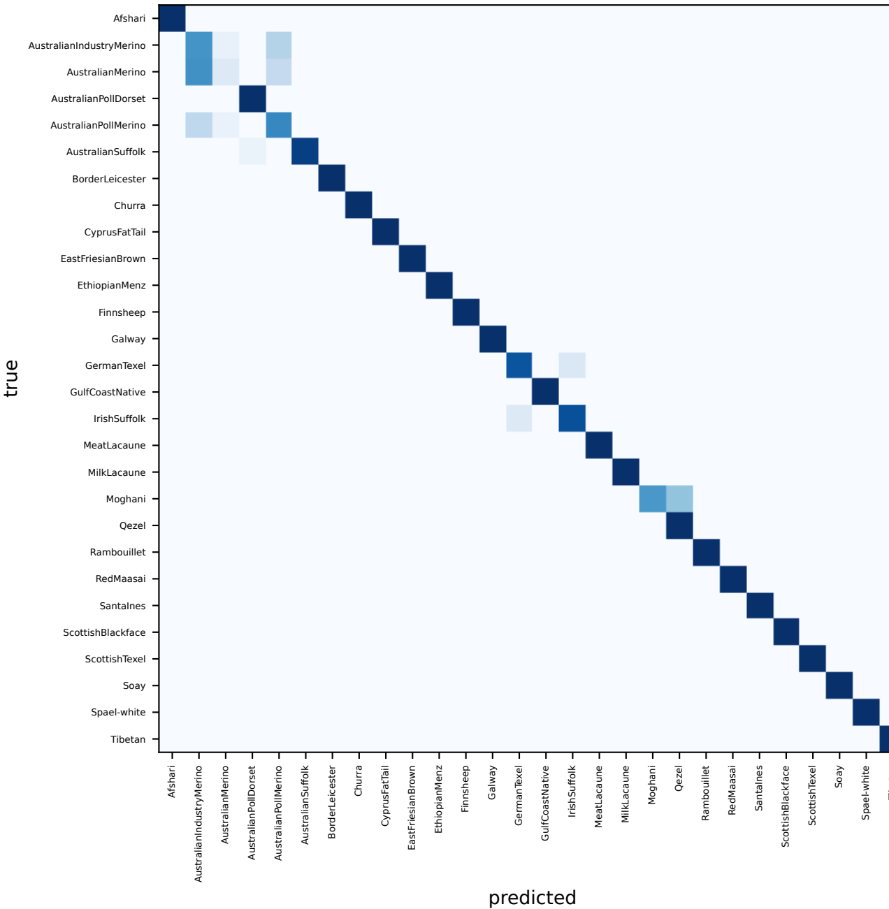
Contrastive emb=3 (KNN k=3) MacroF1=0.915
