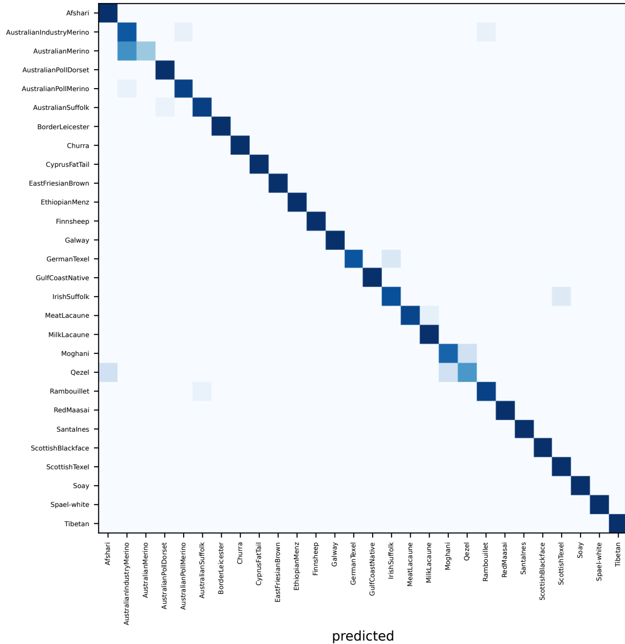
Random Forest MacroF1=0.933
