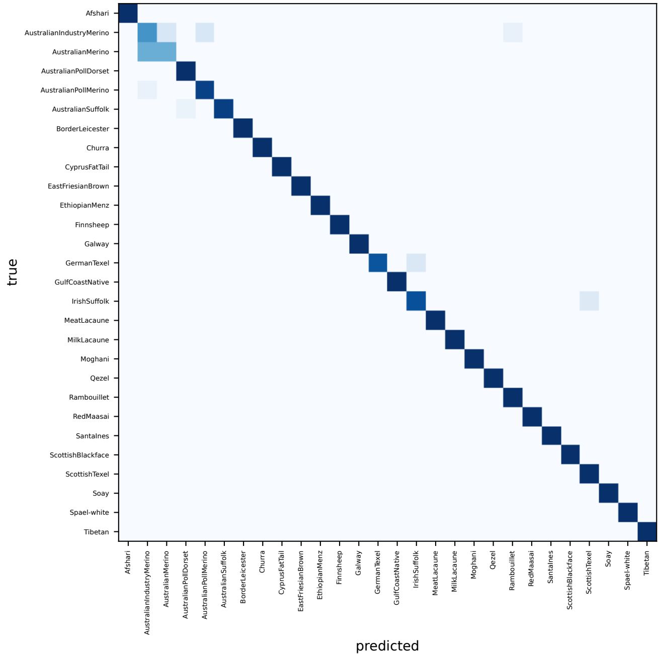
RQ1 sheep cross-species — locked-test confusion matrices (278 animals) VMGP d=96 MacroF1=0.955
