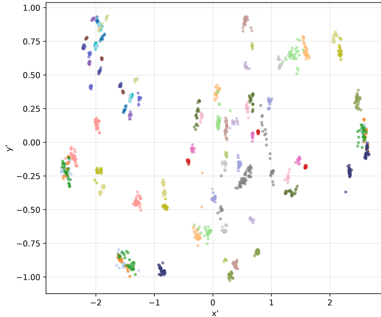
Equal Earth projection of S^2
