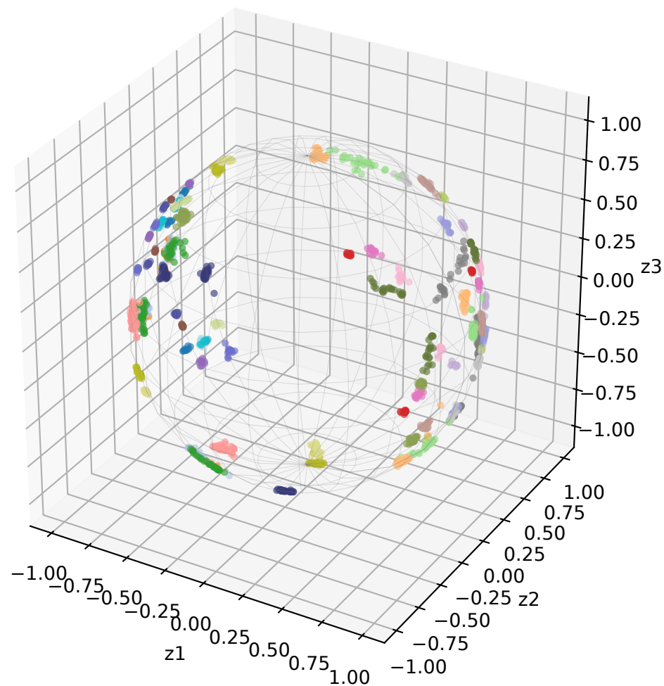
Contrastive embeddings on S^2 (validation folds)
