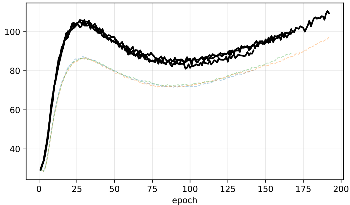
KL divergence (nats/sample)
