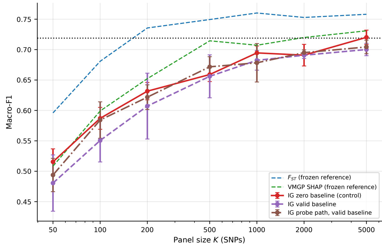
Valid-baseline Integrated Gradients under the frozen Random Forest evaluator
