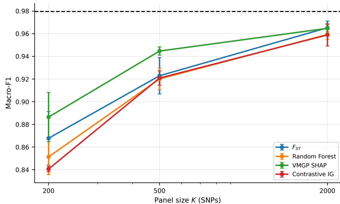
VMGP retrained on the panel ( S_{\text{full}} = 0.9796 )
