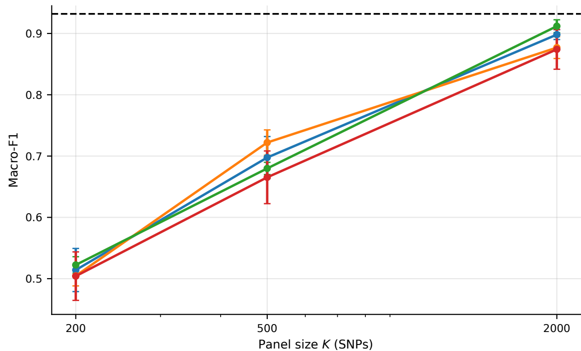
Contrastive model retrained on the panel ( S_{\text{full}} = 0.9320 )
