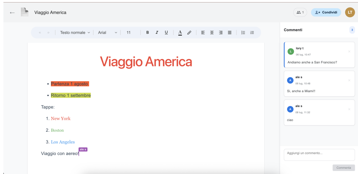
Figure 9: The document.
