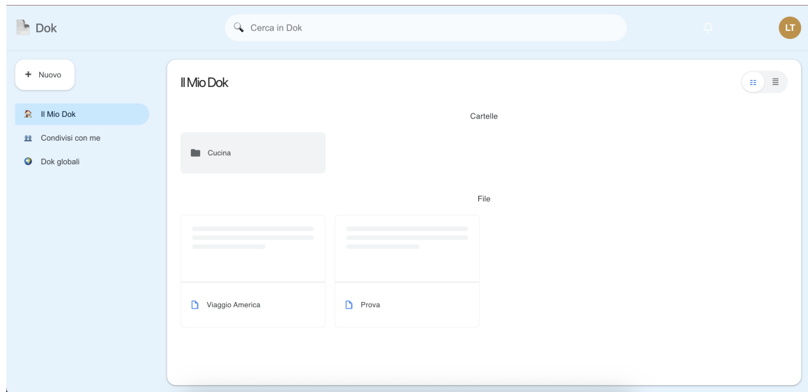
Figure 8: Dashboard.
