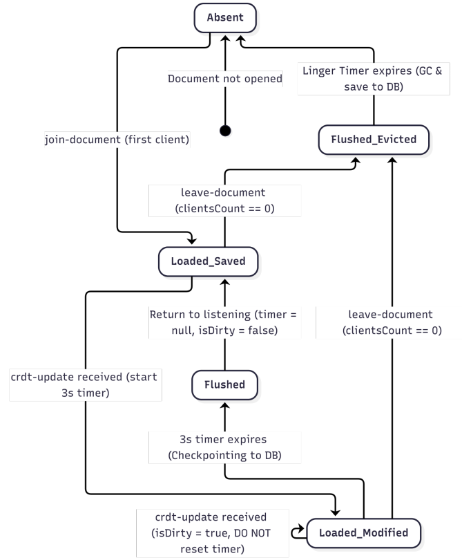
Figure 5: Document lifecycle inside server.
