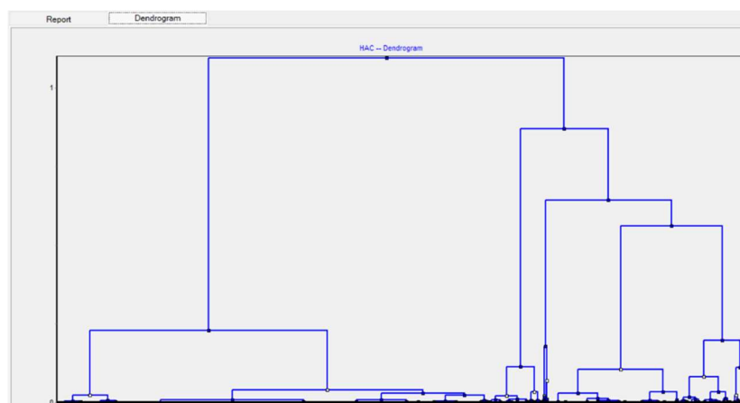
Figure 9 : Dendrogramme
