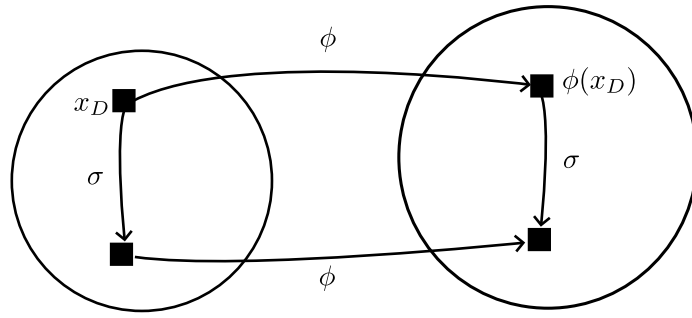
Figure 6: Deterministic part of the homomorphism
