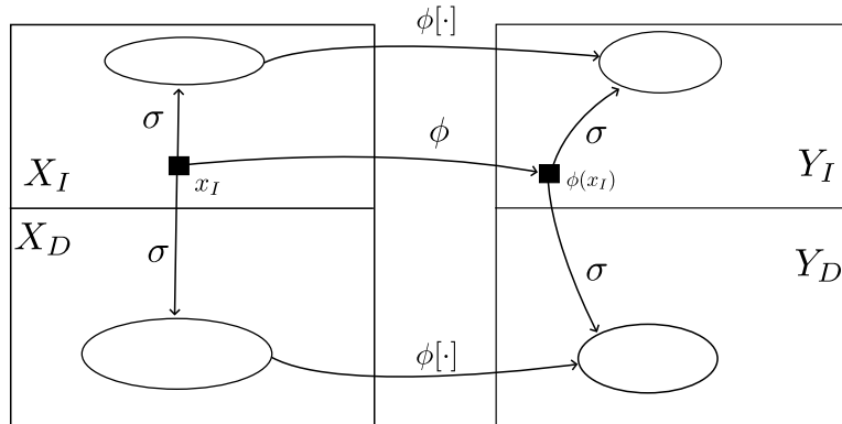
Figure 5: Initial part of the homomorphism
