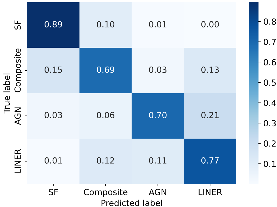
XGBClassifier Confusion Matrix (Rebalanced)
