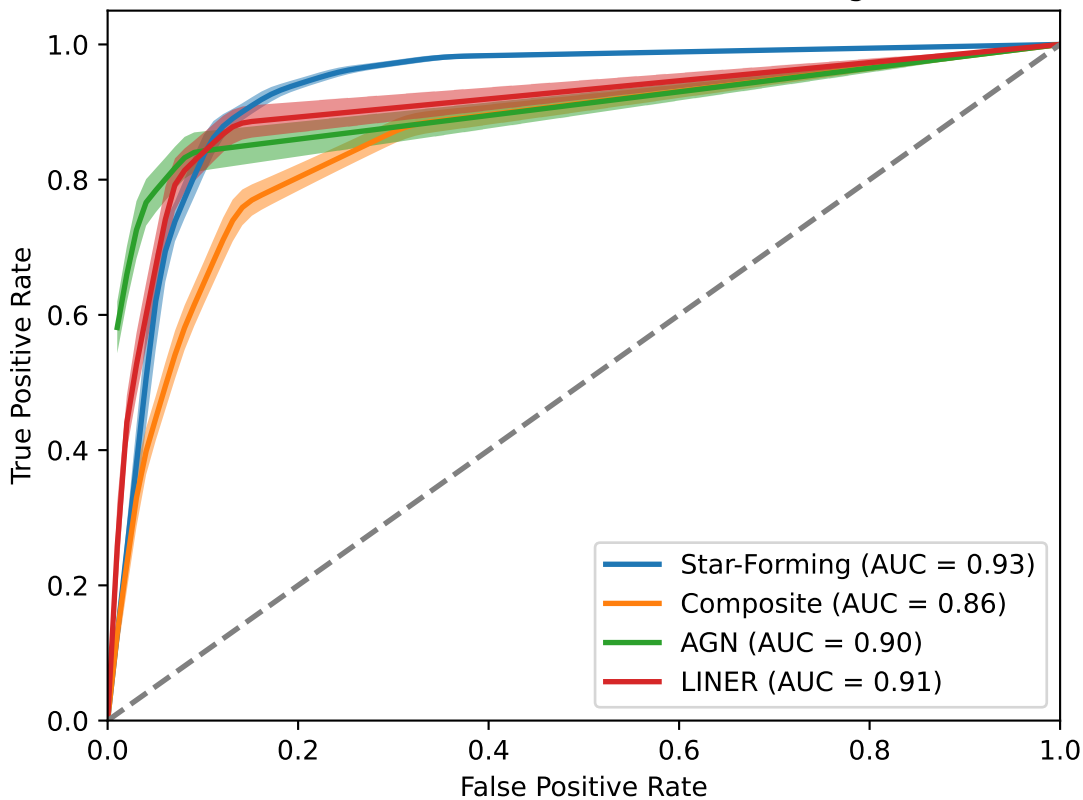
KNN ROC Curve with Default Settings
