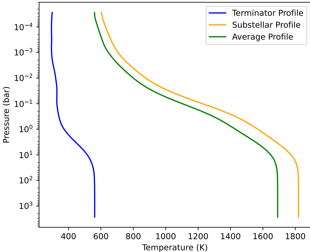
PT Profile LHS1478
