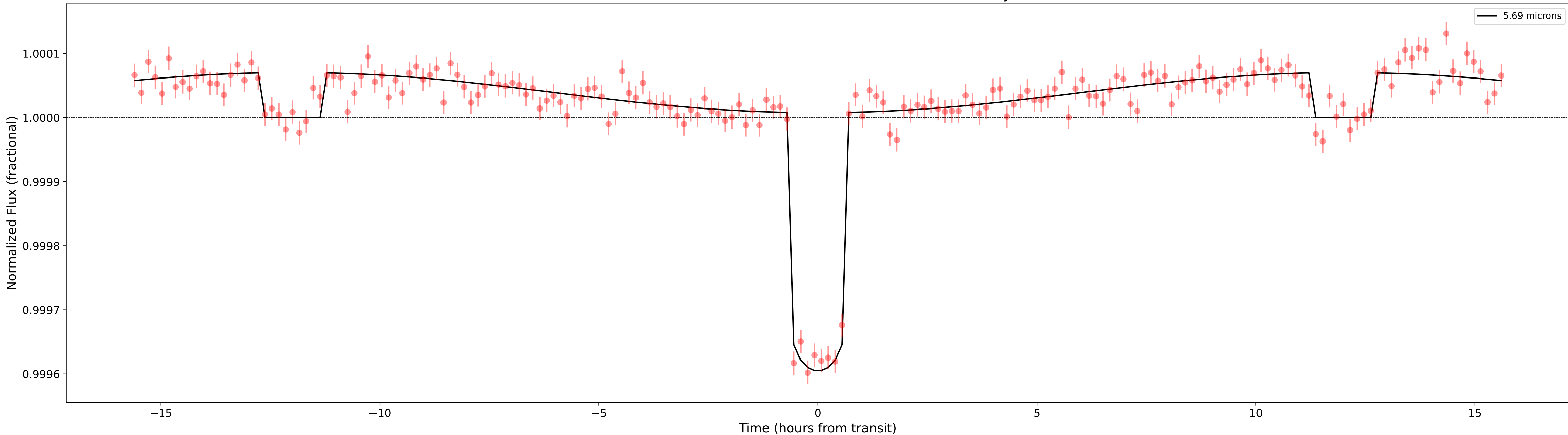
Phase curve of TOI1416b; N=32, total time=32.00 days
