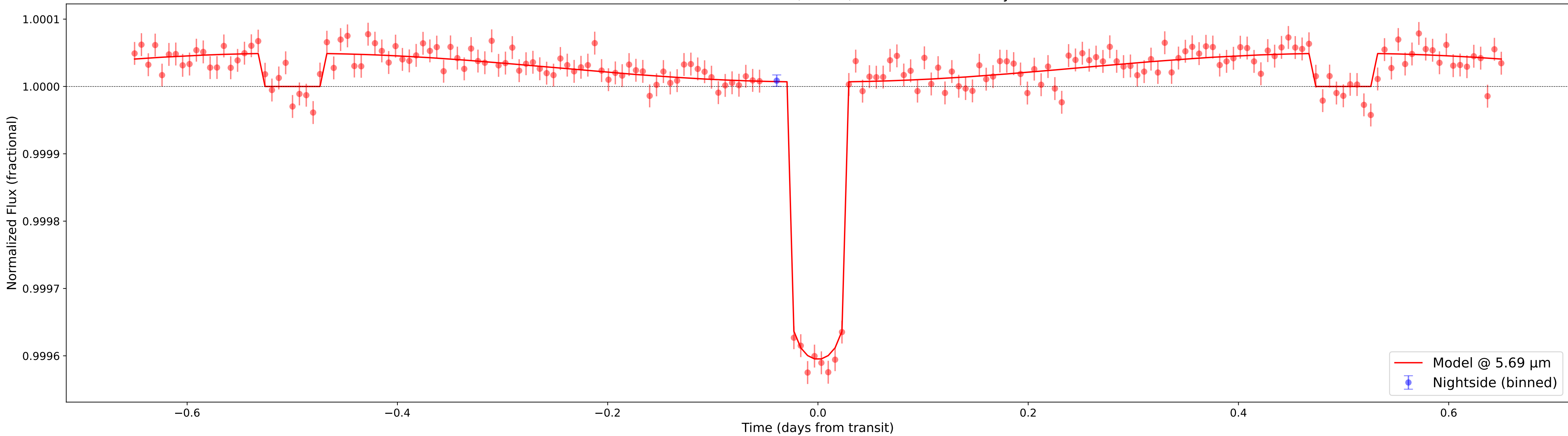
Phase curve of TOI1416b; N=36, total time=36.00 days
