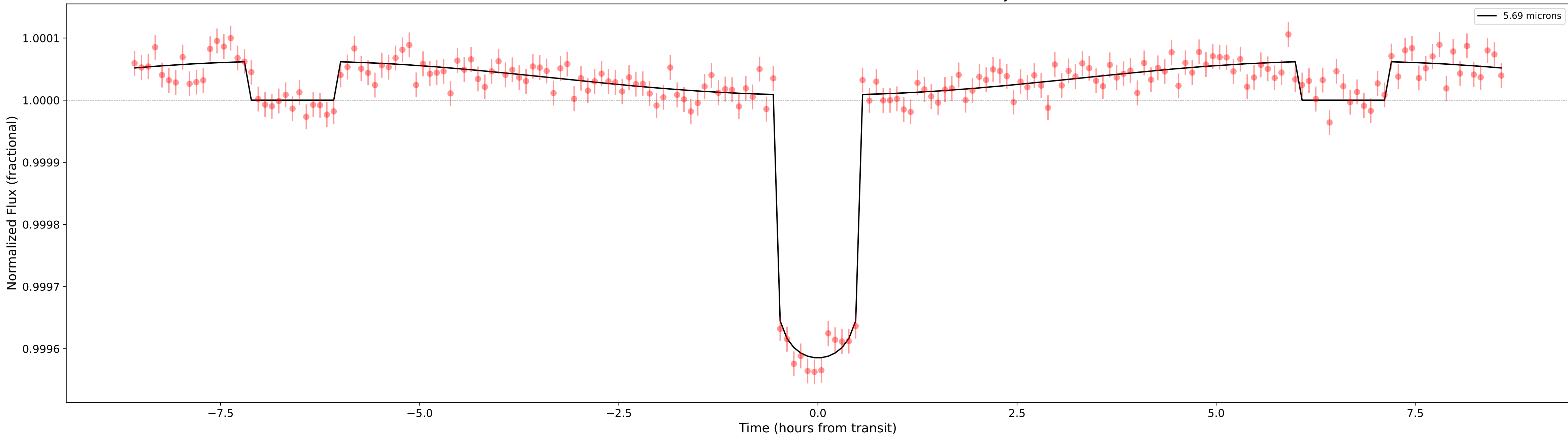
Phase curve of TOI1807b; N=32, total time=17.60 days
