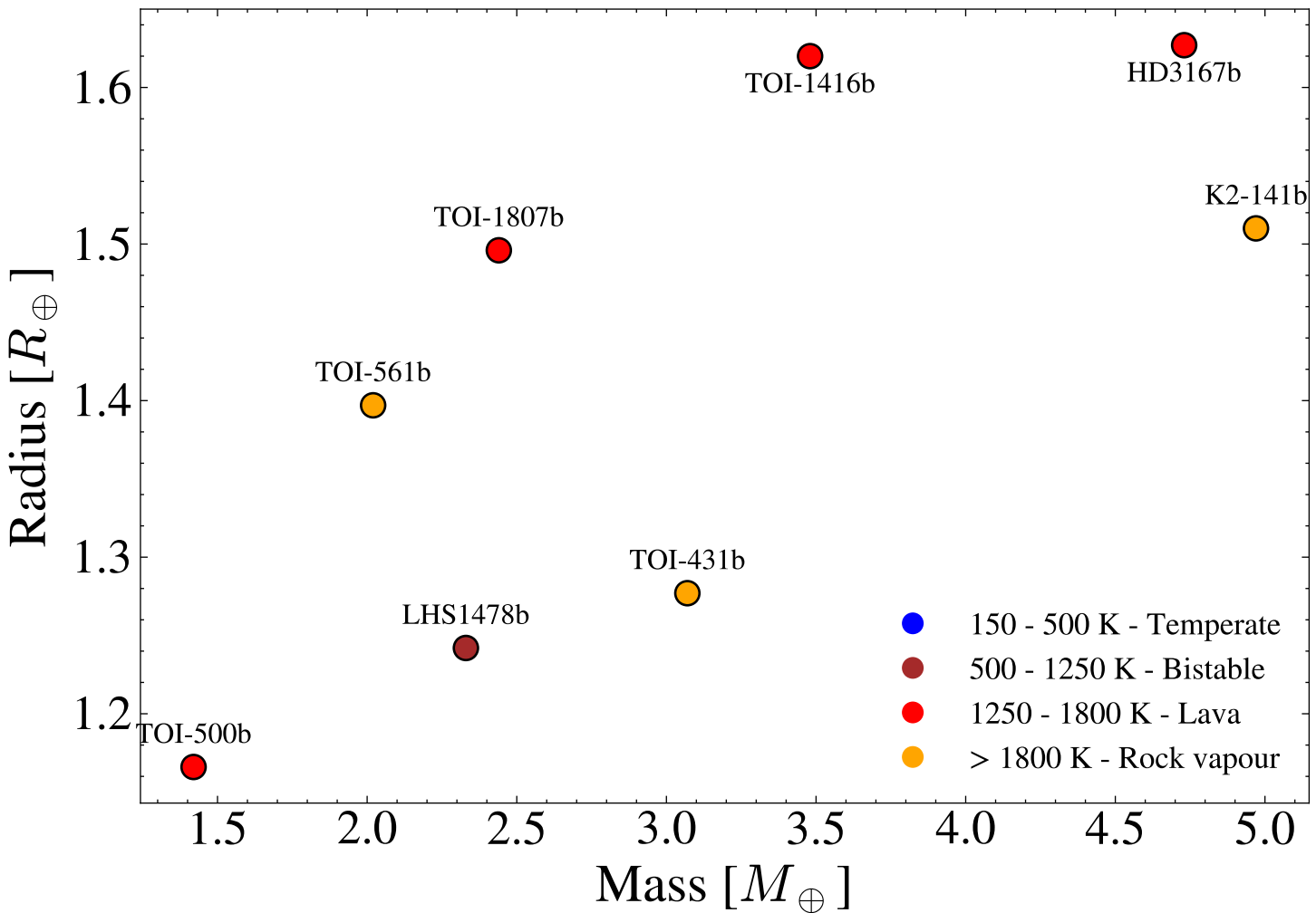
Planet mass vs radius
