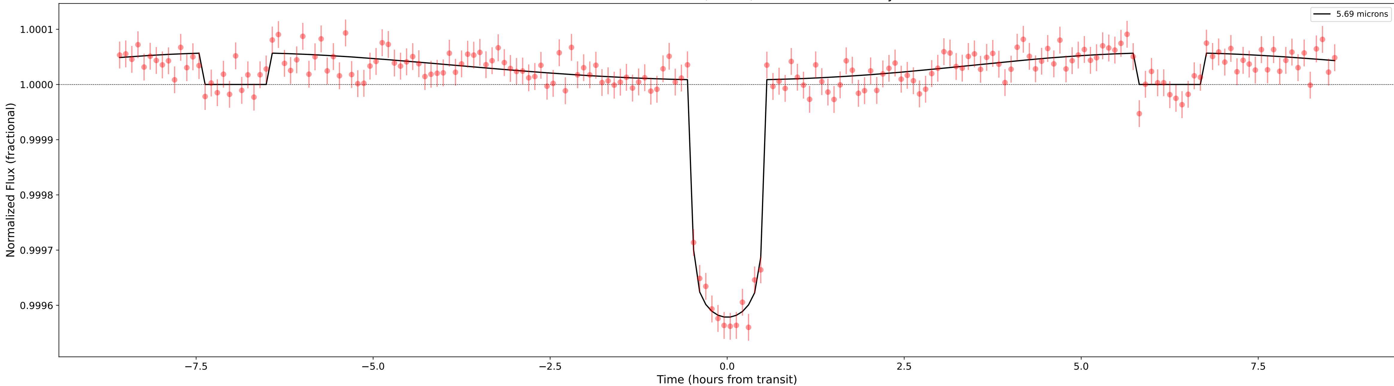
Phase curve of TOI500b; N=36, total time=19.80 days
