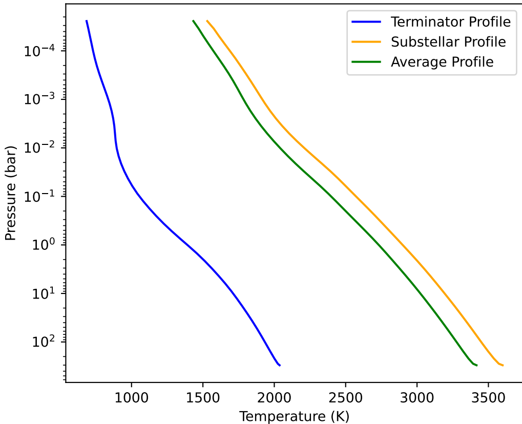
PT Profile HD3167
