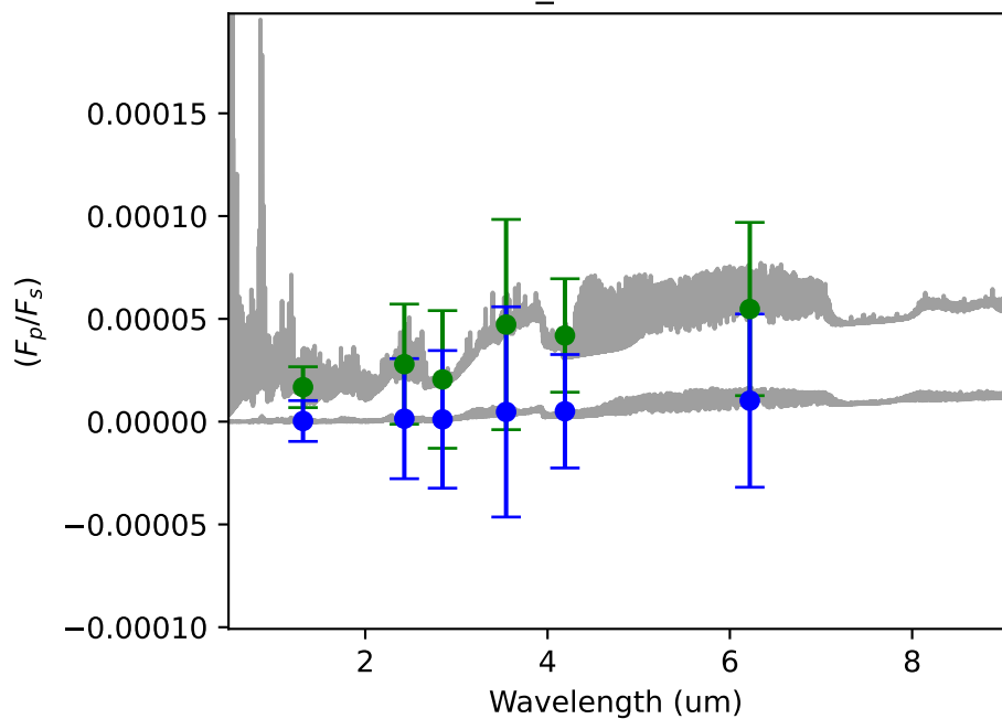
TOI1807_1 - 66.00 hours
