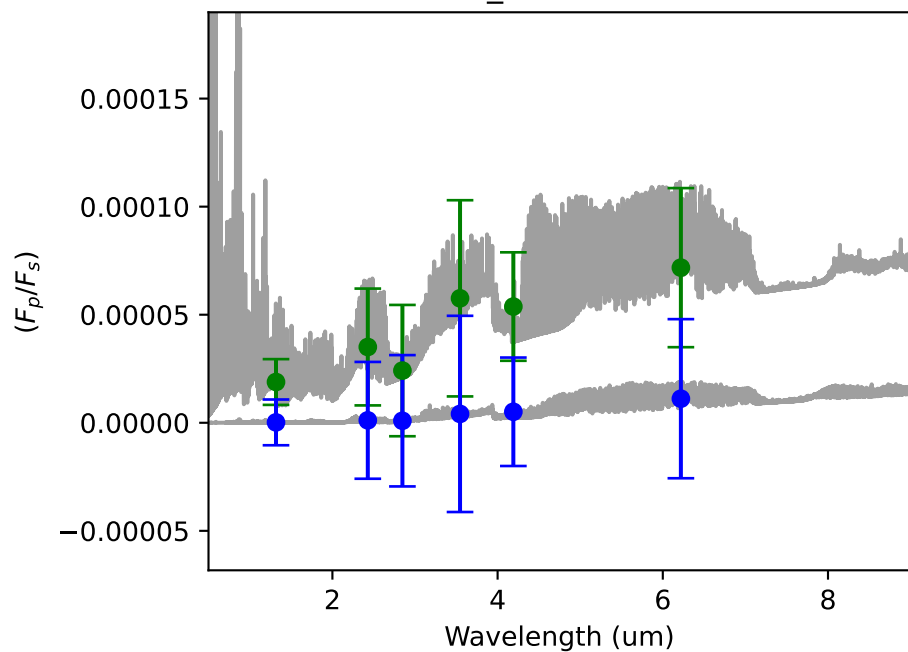
TOI1416_1 - 120.00 hours
