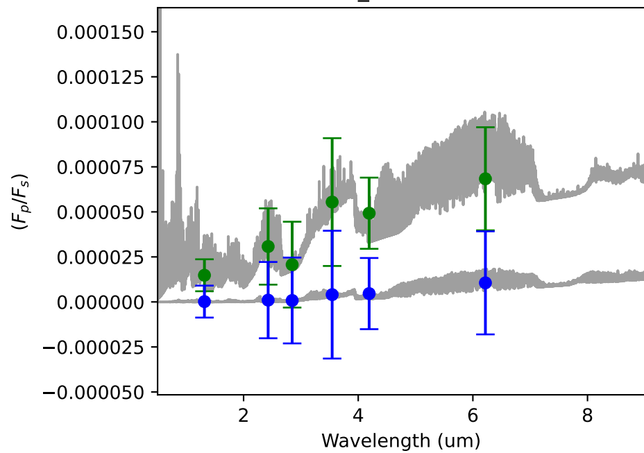
TOI1807_1 - 66.00 hours
