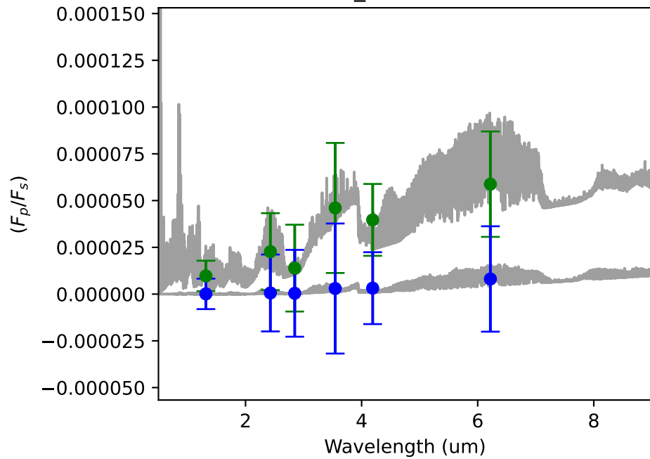
TOI1416_1 - 120.00 hours
