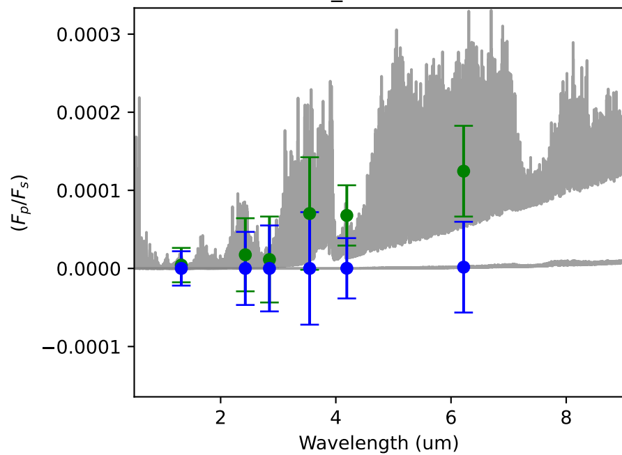
TOI500_1 - 66.00 hours
