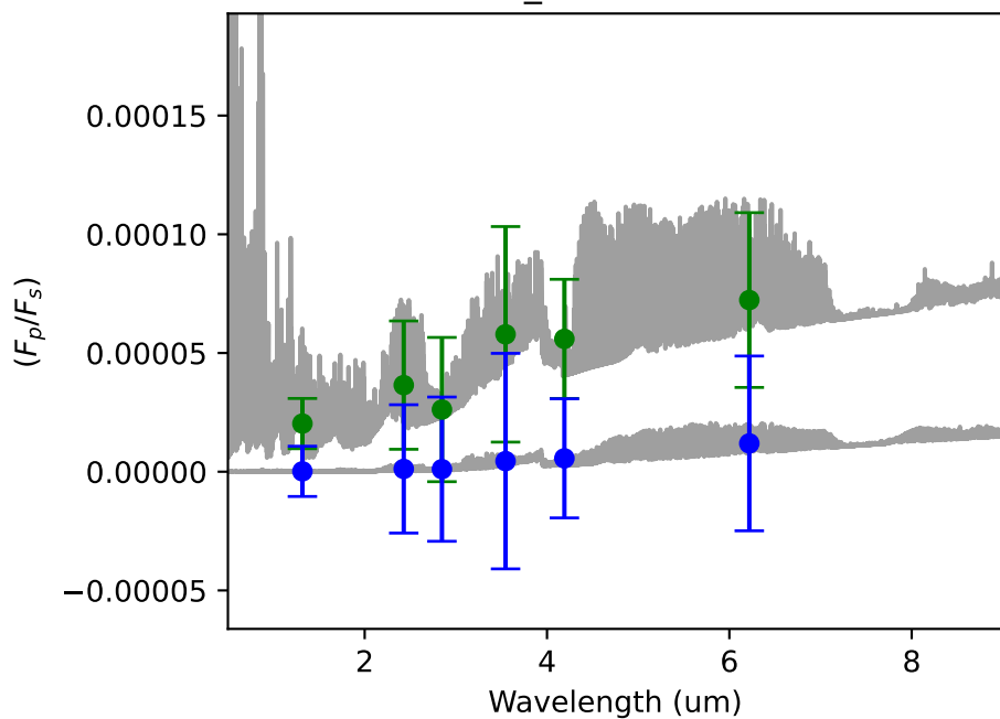
TOI1416_10 - 120.00 hours
