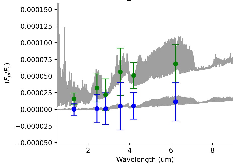
TOI1807_10 - 66.00 hours
