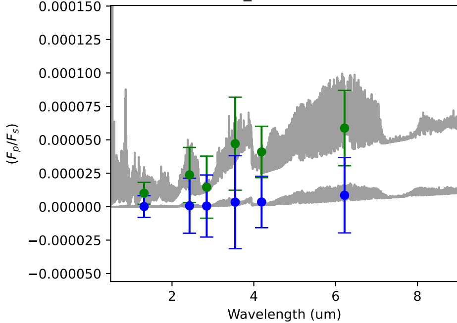
TOI1416_10 - 120.00 hours
