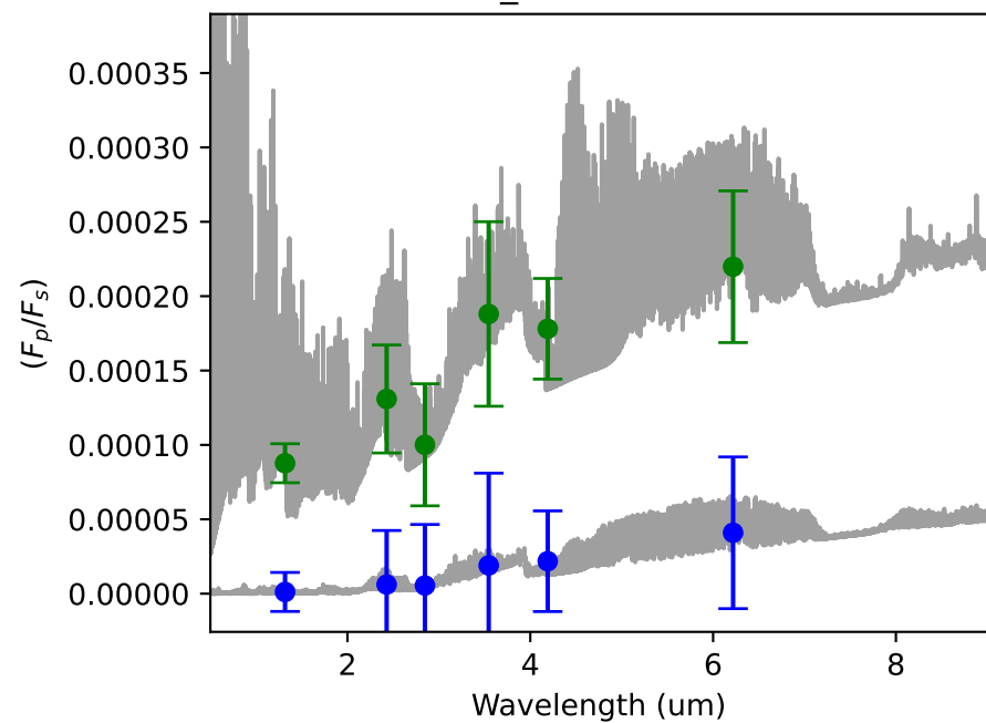
TOI431_10 - 58.80 hours
