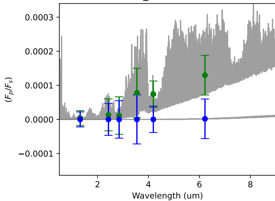
TOI500_10 - 66.00 hours
