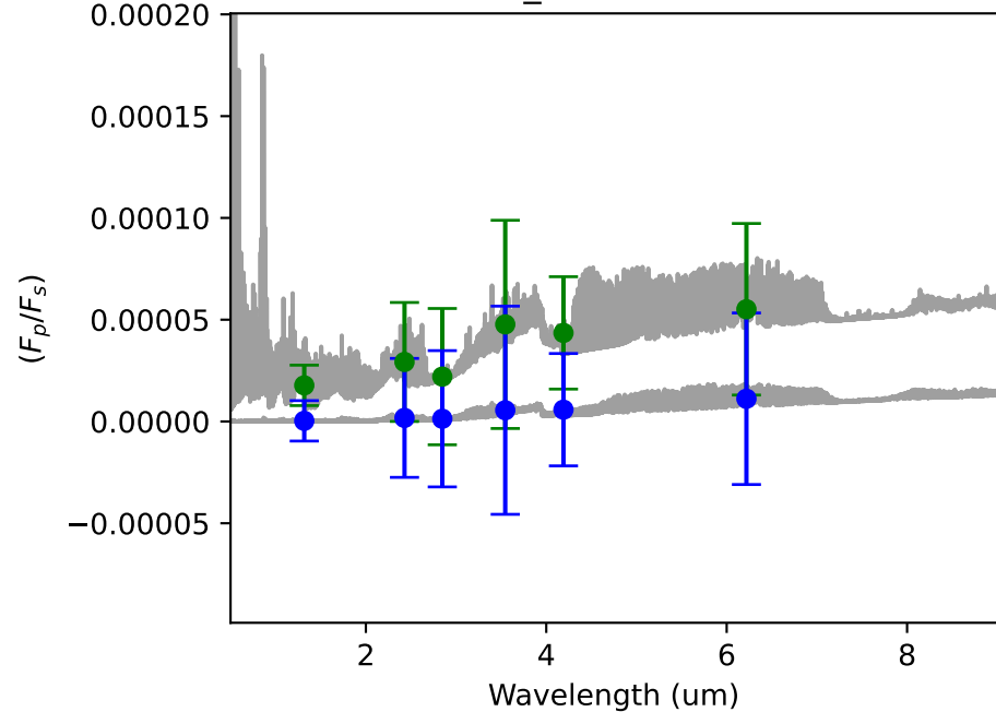
TOI1807_10 - 66.00 hours
