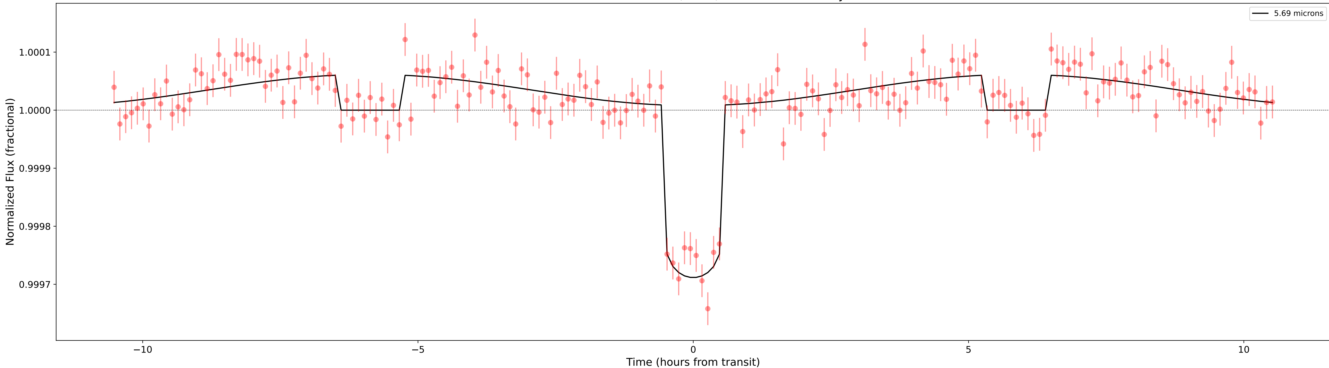
Phase curve of TOI431b; N=9, total time=4.41 days
